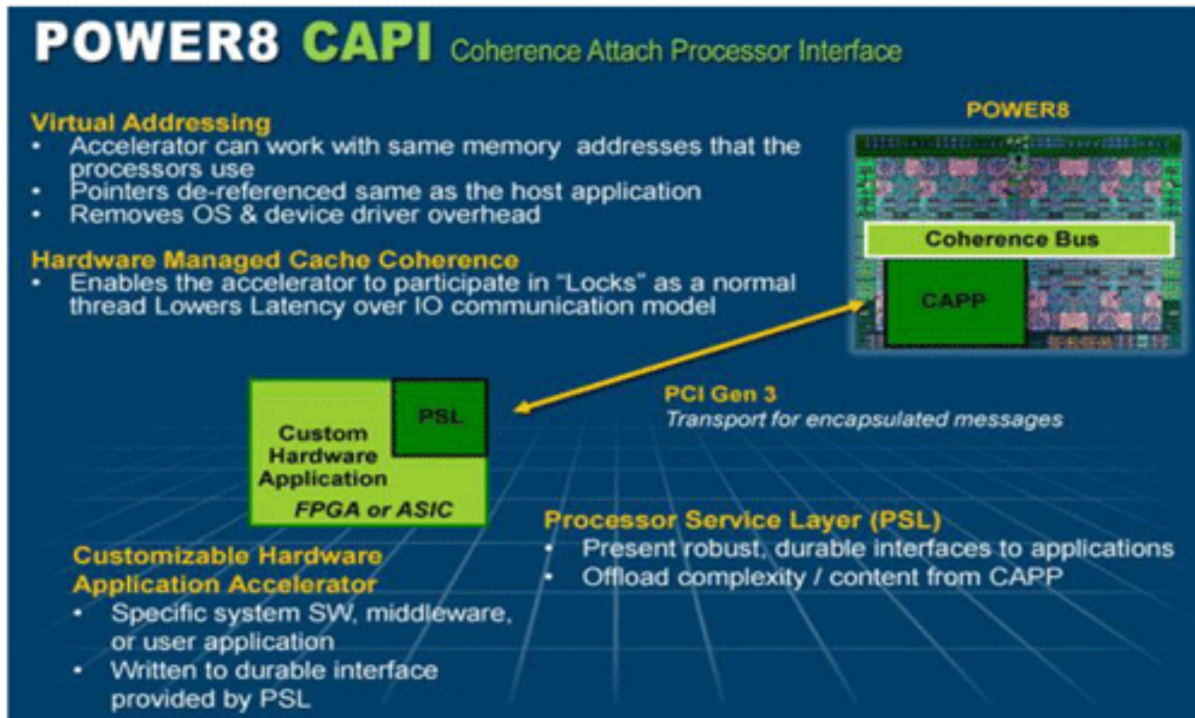
Figure 1 –Key Xeon/POWER Microprocessor/Subsystem Differentiators
